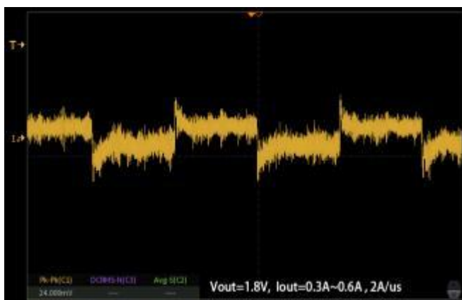
Vout=1.8V Dynamic Response
