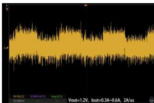
Vout=1.2V Dynamic Response
